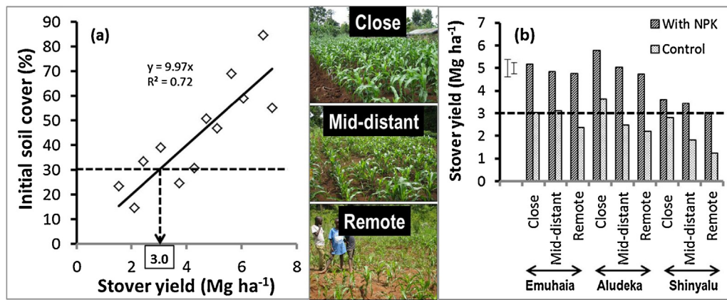
Fig. 1. Relationship between maize stover yield and soil cover at the start of the cropping seasons in Central Kenya (adapted from Guto et al., 2011) (a), and maize stover yields for different field types in three districts of Western Kenya with and without fertilizer (adapted from Vanlauwe et al., 2006) (b). The error bars in (b) are standard errors of the difference to compare stover yields within site, the left bar for the plots with fertilizer and the right bar for the control plots. The horizontal dashed line represents the 30% soil cover limit required for CA. Photographs in the centre give an impression of the maize plots close to harvest on the different field types in Central Kenya.
