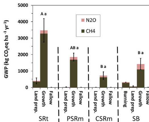
Fig. 5. Total GWP ( \text{CH}_4 and \text{N}_2\text{O} ) of all straw treatments encompassing land preparation, growth and fallow periods as well as computed GWP of straw burning during (a) 2015WS and (b) 2016DS. Values represent the mean of three replicates \pm combined standard error (SE). The different upper case letters reflect a significant difference ( p < 0.05 ) in GWP \text{CH}_4 ; while different lower case letters reflect a significant difference ( p < 0.05 ) in GWP \text{N}_2\text{O} (using Tukey-Kramer test) during the growth period only. SRT – straw retained; PSRm – partial straw removal; CSRm – complete straw removal; SB – straw burned.
