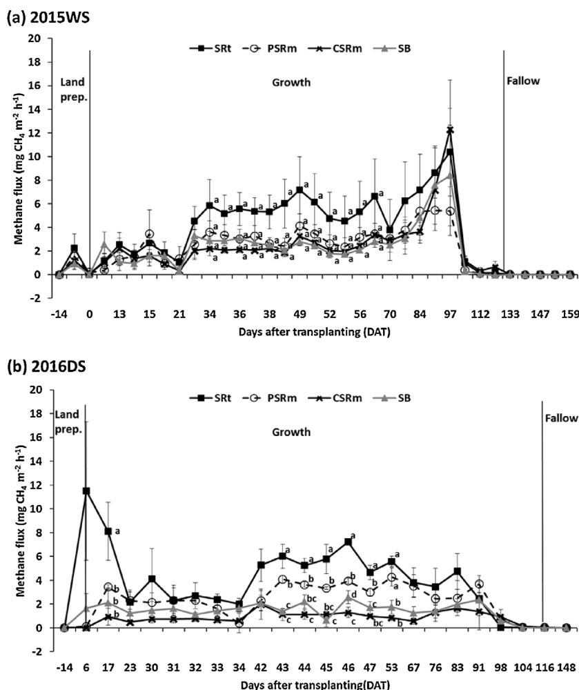
Fig. 3. Seasonal variations in CH 4 flux during (a) 2015WS and (b) 2016DS cropping periods. Values represent the mean of three replicates \pm standard error (SE). During each sampling period, the numbers followed by same letters are not significantly different by LSD test at 0.05 level. SRT – straw retained; PSRm – partial straw removal; CSRm – complete straw removal; SB – straw burned.
