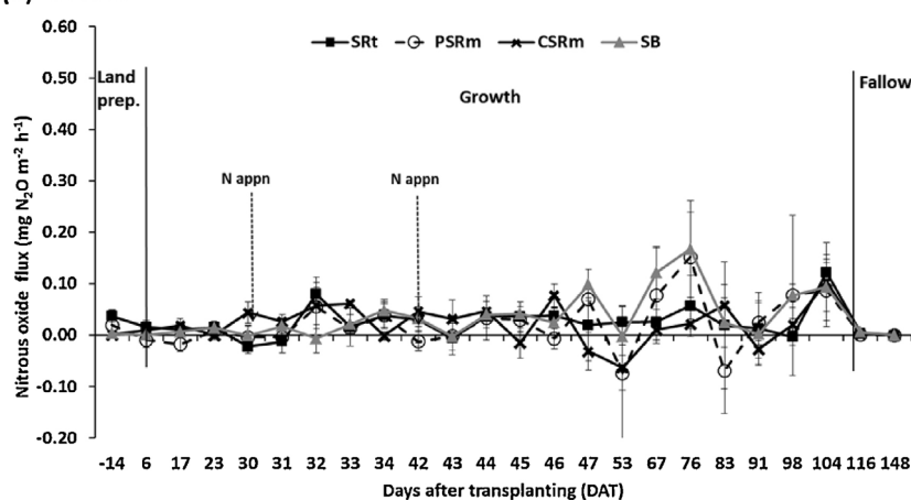
Fig. 4. Seasonal variations in \text{N}_2\text{O} flux during (a) 2015WS and (b) 2016DS cropping periods. Values represent the mean of three replicates \pm standard error (SE). SRT – straw retained; PSRm – partial straw removal; CSRm – complete straw removal; SB – straw burned.
