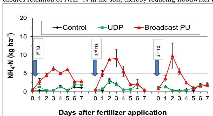
Figure 1. Dynamics of floodwater ammonium (NH 4 -N) under control (N 0 ), broadcast PU and urea deep placement (UDP) at Bangladesh Rice Research Institute (BRI) during dry season ( Boro ) 2015. TD-1, TD-2, TD-3 represent first, second and third topdressing of urea, respectively. Deep placement was done at a time during first topdressing of urea; vertical bars represent standard error (n=3)
