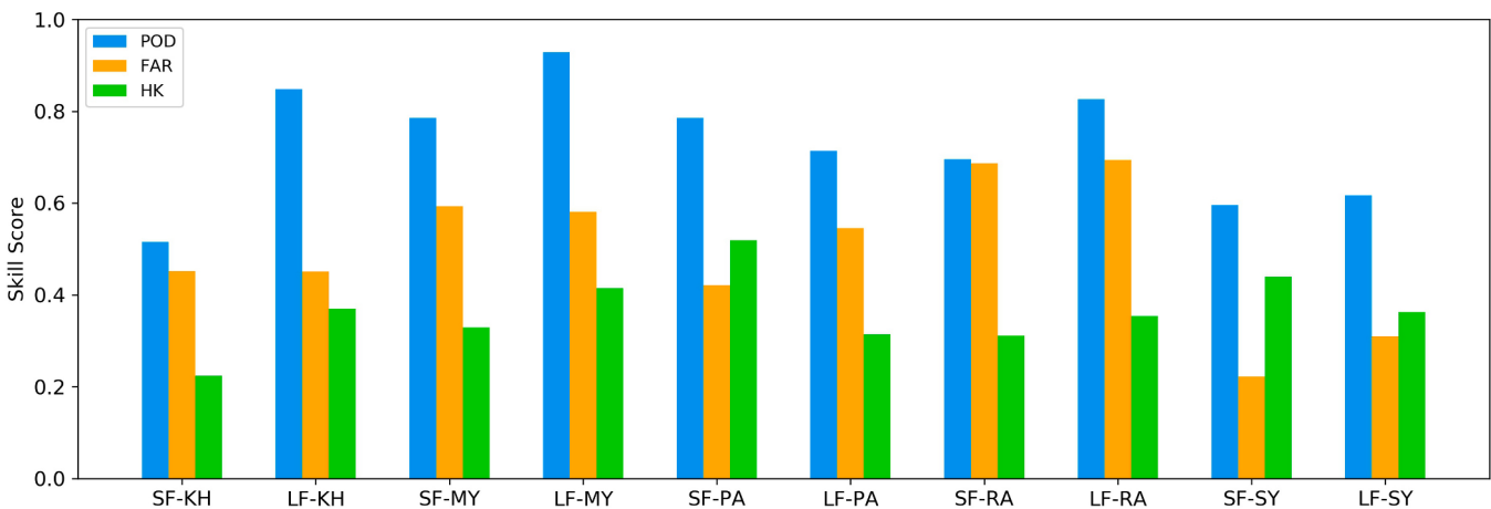
Fig. 4. Scientific (SF) and local forecast (LF) skills compared to in situ observation dataset for the five study locations: Khulna (KH), Mymensingh (MY), Patuakhali (PA), Rajshahi (RA), and Sylhet (SY).
