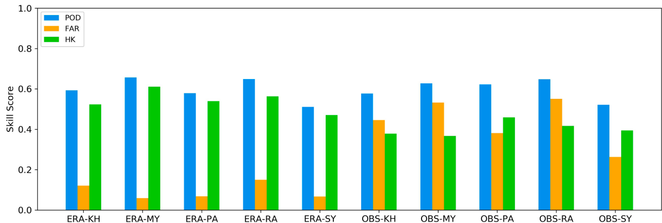
Fig. A.3. Same as Fig. 2 but for rainfall higher than 1 mm/d.
