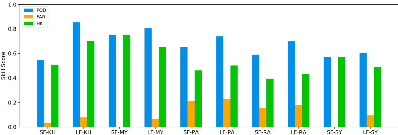
Fig. 3. Scientific (SF) and local forecast (LF) skills compared to the ERA5 dataset for the five study locations: Khulna (KH), Mymensingh (MY), Patuakhali (PA), Rajshahi (RA), and Sylhet (SY).
