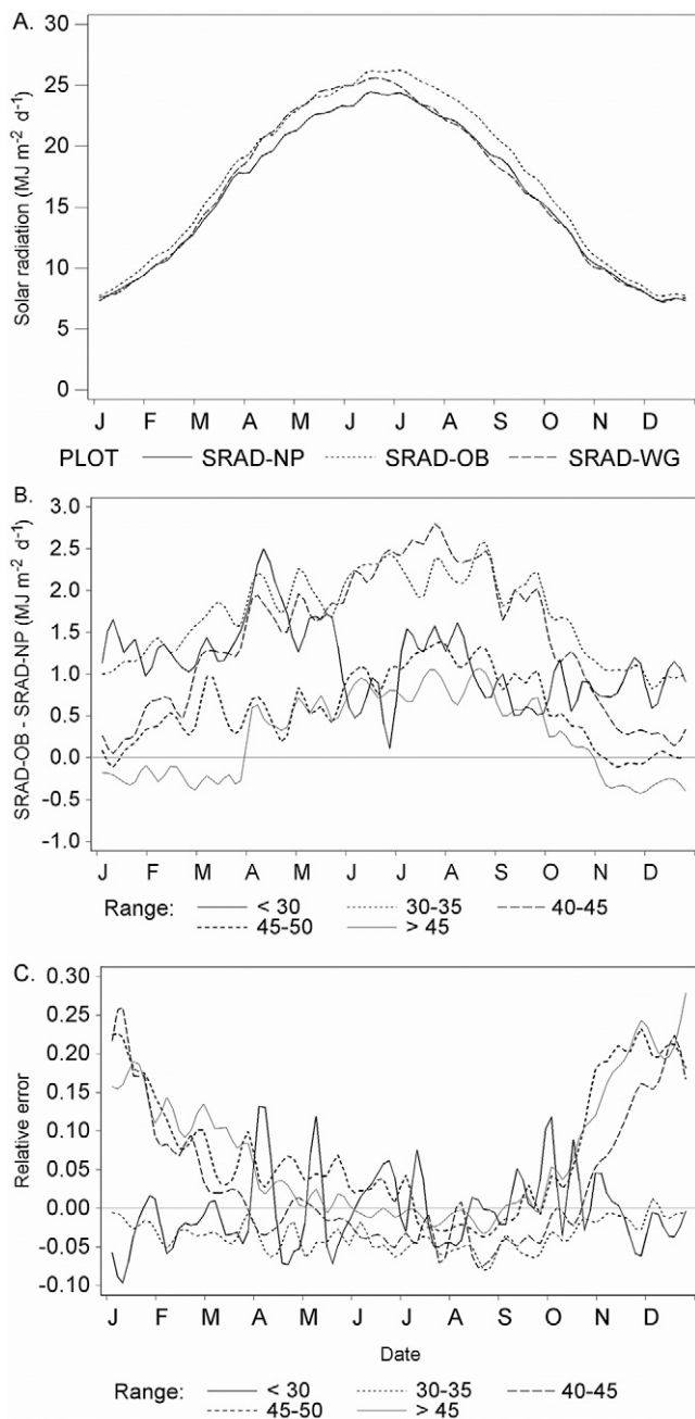
Fig. 5. Annual variation in solar radiation based on 7-d averages. (A) Daily means across all locations for SRAD OB , SRAD NP and SRAD WG . (B) Mean difference between SRAD OB and SRAD NP for five latitude bands from less than 30°N to greater than 45°N. C. Relative error [(SRAD NP - SRAD OB )/SRAD OB ] for the five latitude bands.
