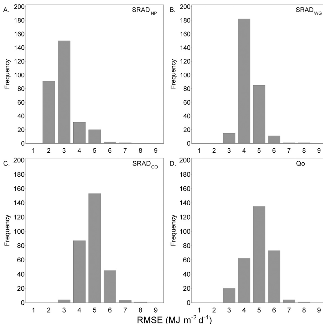
Fig. 3. Root mean square errors (RMSE) for prediction of observed solar radiation from the four other sources. (A) SRAD_{OB} vs. SRAD_{NP} . (B) SRAD_{OB} vs. SRAD_{WG} . (C) SRAD_{OB} vs. SRAD_{CO} . (D) SRAD_{OB} vs. Q_0 .
