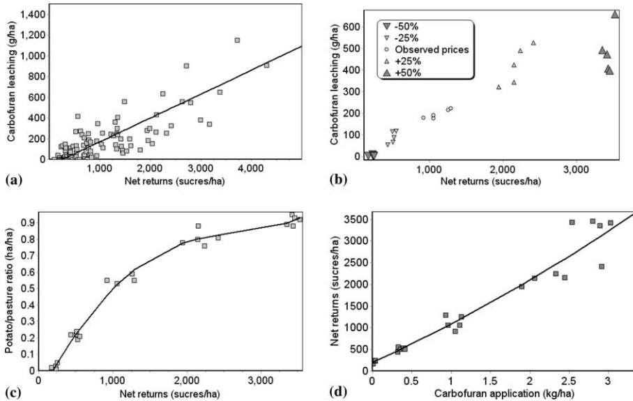
Fig. 5. The relation between net returns and carbofuran leaching under different potato price regimes (1800 Sucre \approx 1 US$). (a) The variation in net returns and carbofuran leaching as a consequence of spatial variability under current price conditions. (b) The simulation results of the base scenario per tradeoff point. (c) The relative importance of potato in the crop rotation as a function of net returns. (d) The effect of carbofuran application on net returns.
