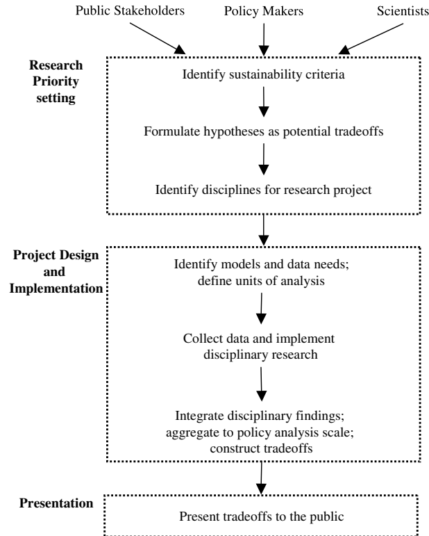
Fig. 1. Tradeoffs analysis research design and implementation process (Crissman et al., 1998a).
