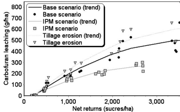
Fig. 8. The effect of IPM and tillage erosion on the tradeoff curve (1800 Sucre \approx 1 US$).
