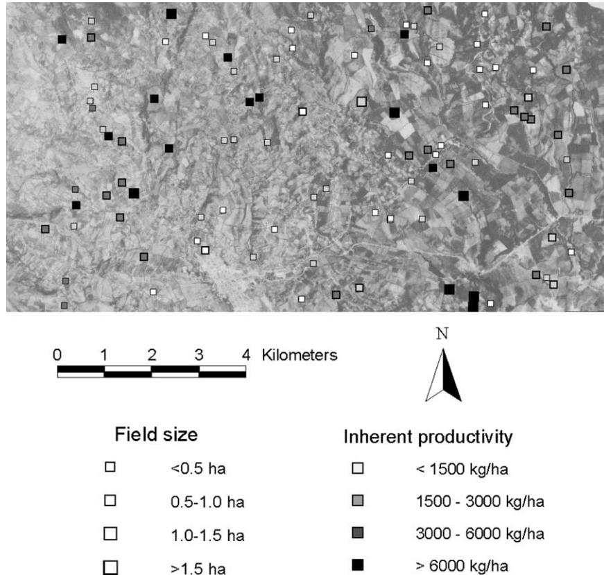
Fig. 4. The location, field size, and the inherent potato production of the sampled fields in the San Gabriel region of Carchi Province, Ecuador.
