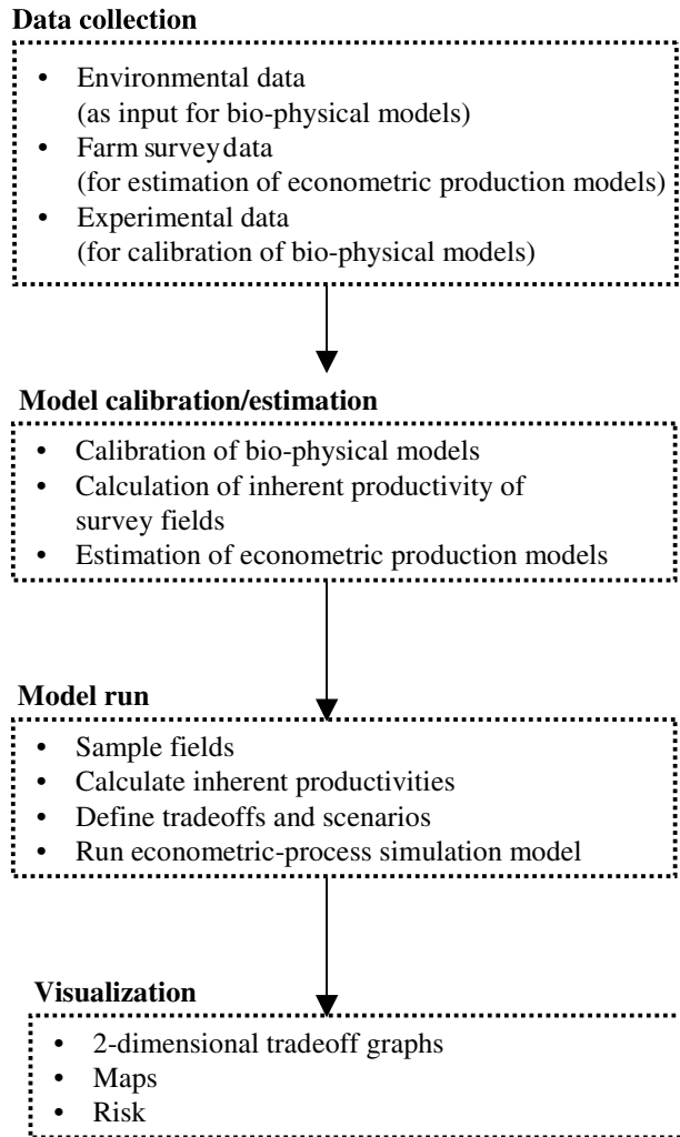
Fig. 3. General framework of the Tradeoff Analysis Model.
