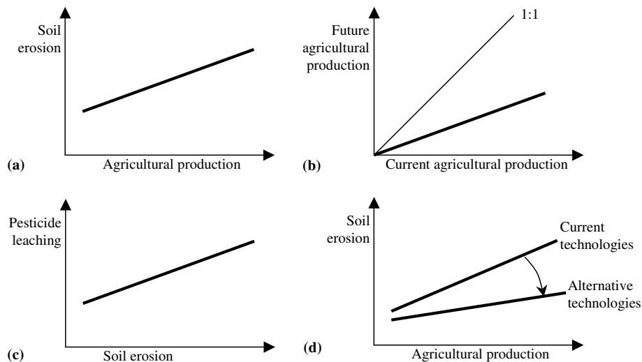
Fig. 2. Examples of possible tradeoff curves. (a) Increased soil erosion when intensifying agricultural systems. (b) The negative effects on future productivity as a result of soil erosion when intensifying current agricultural production. (c) Increased pesticide leaching as a result of increased erosion rates. (d) The impact of alternative (conservation) technologies on the tradeoff curve.
